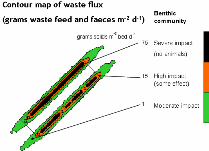
Figure 16. Definition of Severe, High and Moderate impact for the SABBAC zone modelling. There are two rows of cages shown and different colours represent different amounts of waste flux (grams waste feed and faeces depositing on the bed per \text{m}^2 per day)
